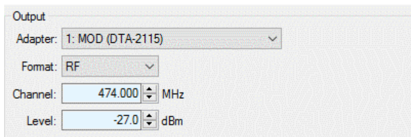
ATSC 3.0 RF output settings
