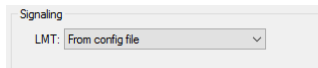
LMT-table generation
